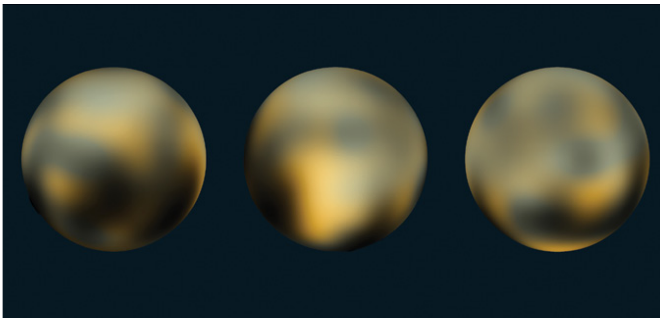
FUZZY VIEW: The surface terrain of Pluto, as seen by the Hubble Space Telescope, varies widely, with a mysterious bright spot appearing in the center view. The New Horizons probe should image Pluto with much more clarity when it arrives next year.
